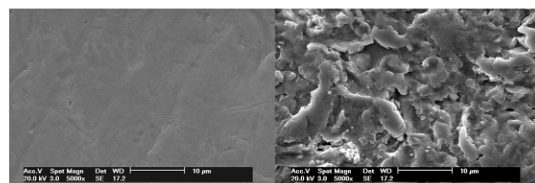
FIGURE 4. The SEM analysis of the CG (A) and EG (B) surfaces at ×5000 magnification.
